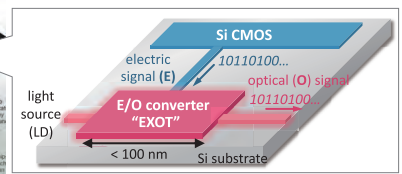
Fig. 2. Optical interconnects using exciton transistors "EXOT" as E/O converters.
